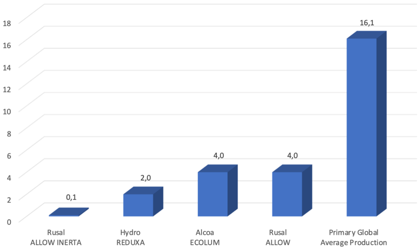
Emissions produced for the production of some primary aluminium brands by major world producers (tCO 2 /t aluminium)
